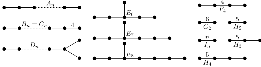
FIGURE 1. Coxeter diagrams corresponding to irreducible Artin groups of finite type. 2
